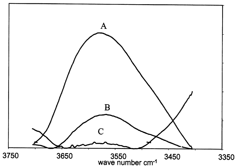
FIGURE 5 Expanded view of APS-treated E-glass fiber from 3750–3400 cm -1 , (a) bare glass fiber, (b) 4.5 \times 10^{-3} mol/L, and (c) 4.5 \times 10^{-2} mol/L.
