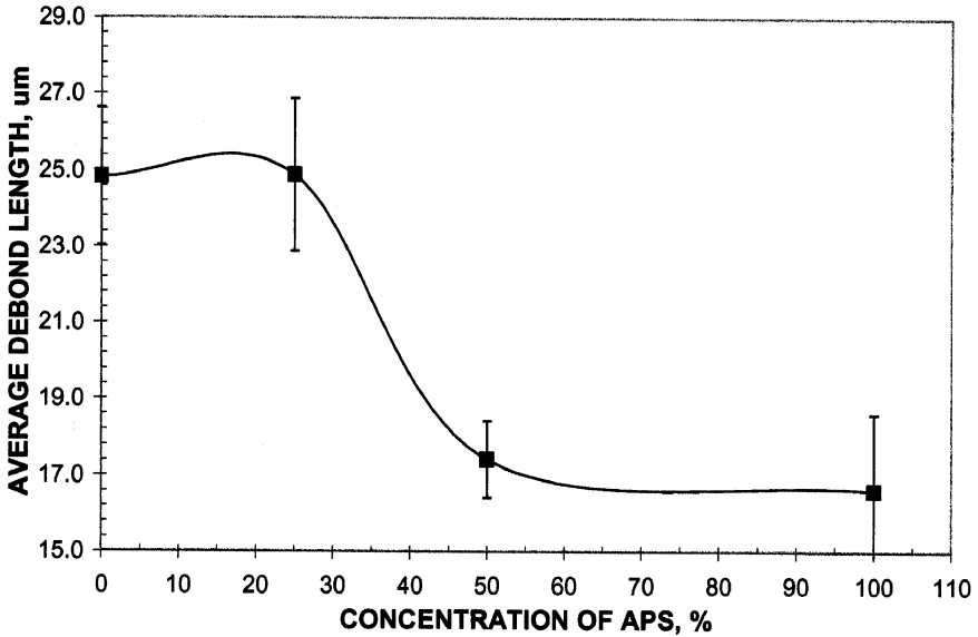
FIGURE 10 Average debond length for E-glass fibers coated with APS and PTMS mixture by aqueous deposition process (error bar represents one standard deviation from the mean and is taken as the standard uncertainty).
