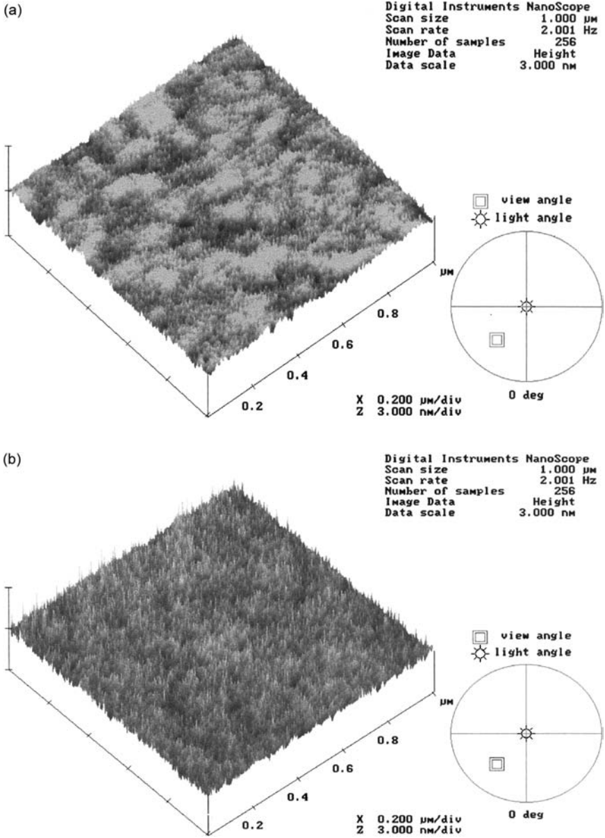
FIGURE 2 (a) TMAFM of APS/PTMS (50 mol% amine) film on silicon wafer; three-dimensional topographic image. (b) TMAFM of bare silicon wafer; three-dimensional topographic image (see Color Plate I).
